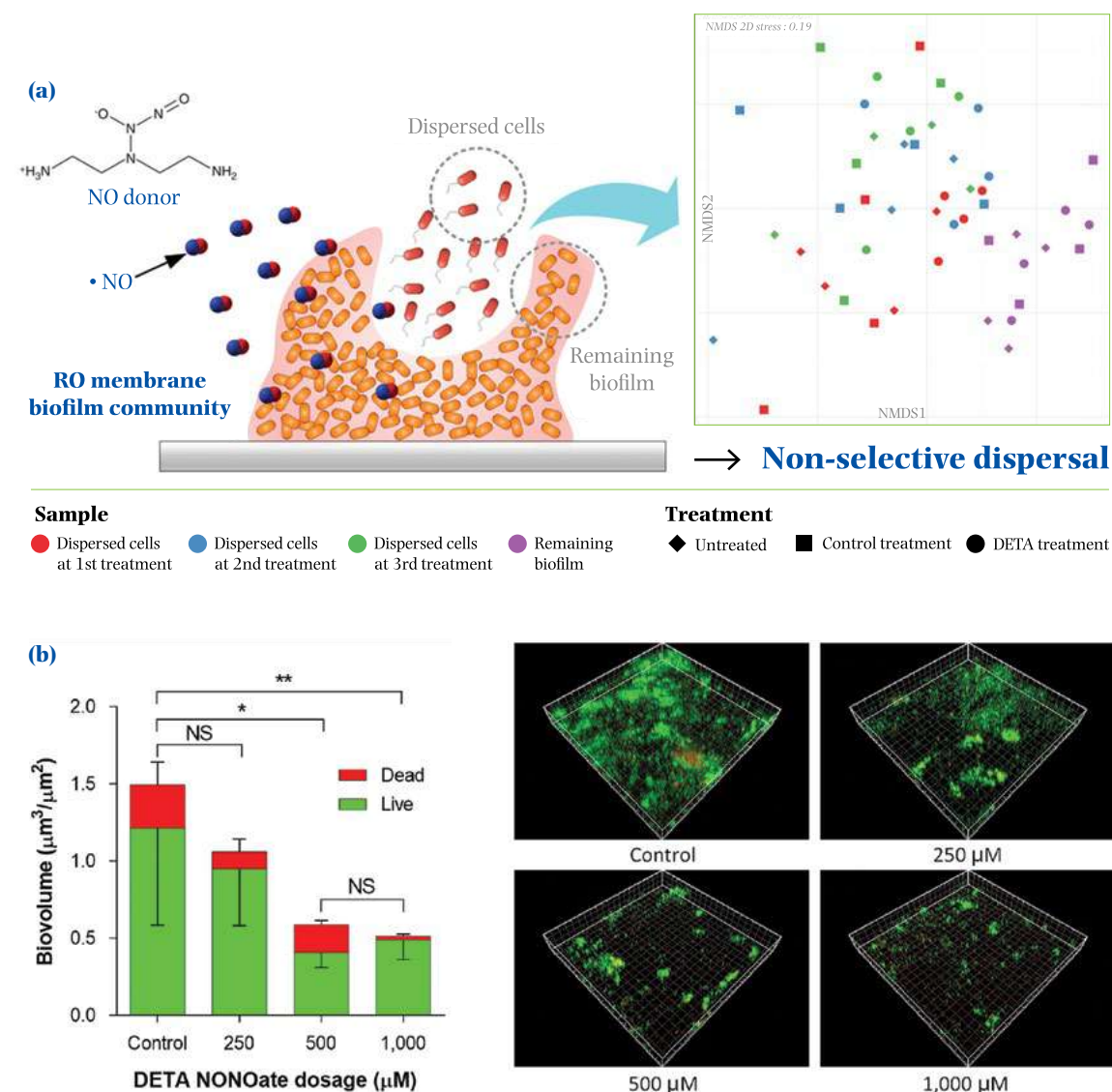
Figure 2: (a) Schematic treatment of RO membrane community with DETA NONOate. Community analysis was carried out and a NMDS ordination plot based on the Bray-Curtis community dissimilarity of the communities was generated. Bacterial communities from remaining or non-dispersed biofilms differed significantly from the dispersed cells (PERMANOVA multivariate test). However, DETA NONOate treatment had no impact on the overall composition of the bacterial community in either dispersed cells or the remaining biofilms, which indicated there were no significant differences between treatment types when considering overall sample types or each different sample type. (b) The biovolume of live and dead cells left on the glass surface of the flow channel after treatment and associated CLSM images. One-way ANOVA and Tukey's post-tests were performed, and significance is represented as: NS (not significant) p_{adj} > 0.05 , * p_{adj} < 0.05 and ** p_{adj} < 0.01 .
